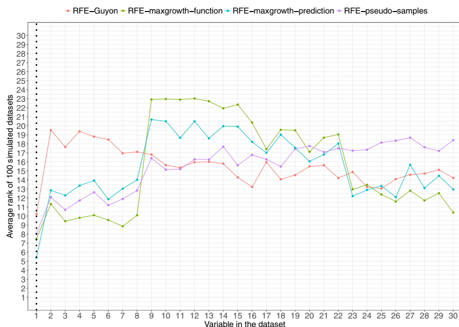
Fig. 5 Scenario 1 results. Average rank by variable and method for the 100 simulated datasets for Scenario 1 (being Variable 1 the relevant variable). Dotted vertical black line represents the variable used to generate the time-to-event variable. The lower the rank, the more relevant the variable is for the specific algorithm
