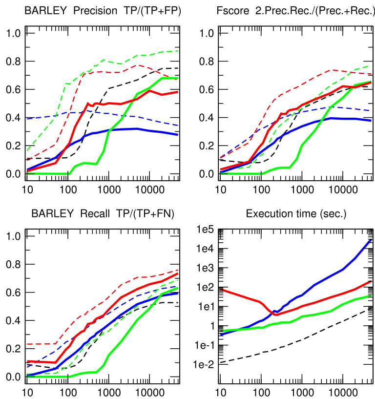
Fig. 5 BARLEY network. [48 nodes, 84 links, 114,005 parameters, Average degree 3.5, Maximum in-degree 4]. Precision, Recall and F-score for skeletons ( dashed lines ) and CPDAGs ( solidlines ). The results are given for Aracne ( black ), PC ( blue ), Bayesian Hill-Climbing ( green ) and 3off2 ( red )
