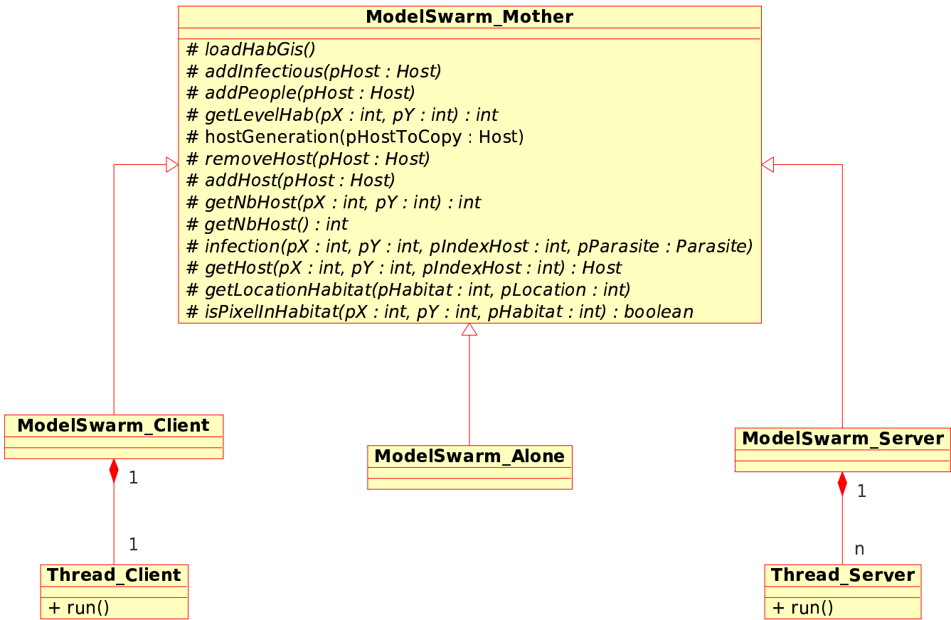
Figure 2 Distributed behavior of our model. Each function acting on the virtual world or on scheduling is in the "Model Swarm" class. These are virtual functions and each behavior is implemented in one of the inheriting classes. "Model Swarm Alone" contains the same functions as the "Model Swarm" class and is applied in a stand-alone use. "Model Swarm Client" and "Model Swarm Server" are called in the case of parallelization. On the server side, a thread is created for each client and communication is done via an established communication protocol (See Additional file 1, section 4). On the client side, each client can focus on a given number of "Host" objects and a thread is created to communicate with the Server component.
