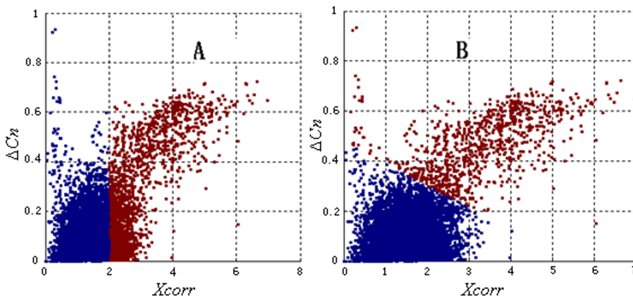
Figure 8 The partitions of k-means clustering before (A) and after (B) normalization (z-score) of the features. Blue and red points represent different clusters. The observations derive from the control dataset. Records with larger Xcorr and \Delta Cn are more likely to be positive results. The partition given by k-means clustering using the observed values is based on Xcorr ; \Delta Cn has no effect. After normalization, the partition is more consistent with the empirical knowledge.
