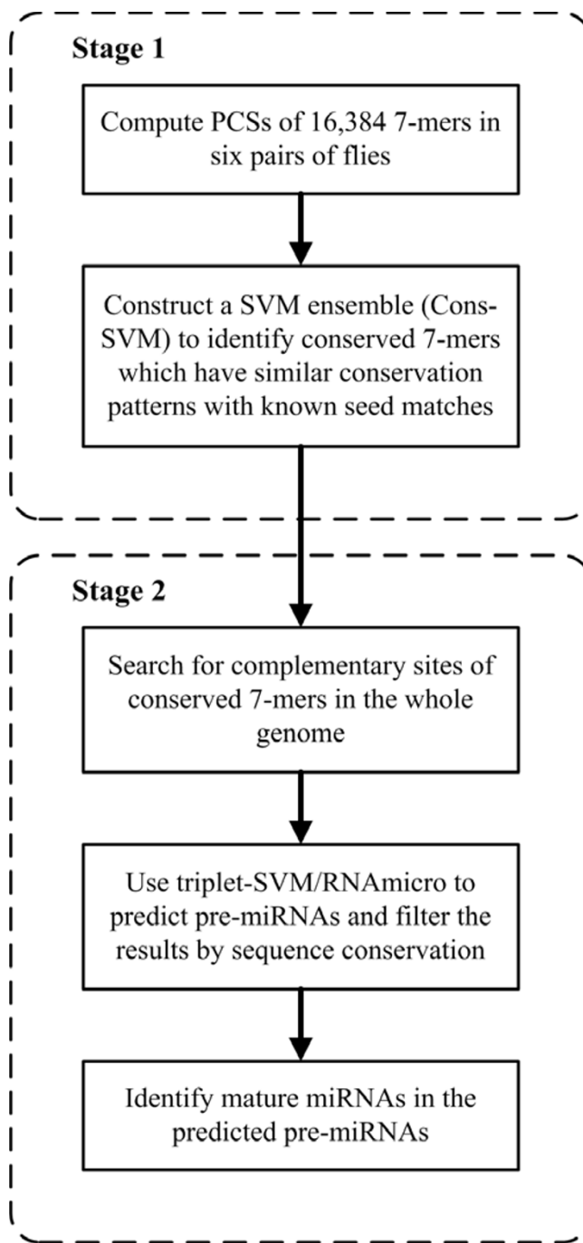
Figure 1 The flowchart of the method. The whole method consists of two stages: in the first stage, conserved 7-mers are identified by considering all 7-mers' conservation patterns in six pairs of flies; in the second stage, pre-miRNAs and mature miRNAs are predicted by adding seed-matching information into published miRNA prediction methods in the whole genome.
