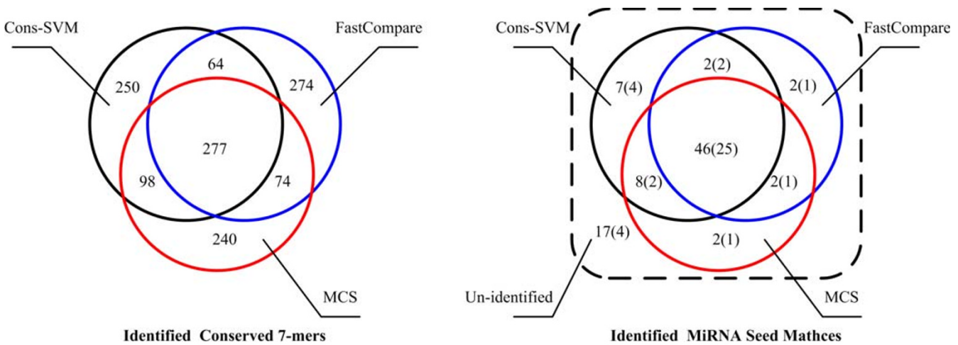
Figure 2 Comparisons of the results using the three methods. The number in each block indicates the corresponding number of 7-mers in that part. The number in the parenthesis indicates the number of reference miRNA families in that block.
