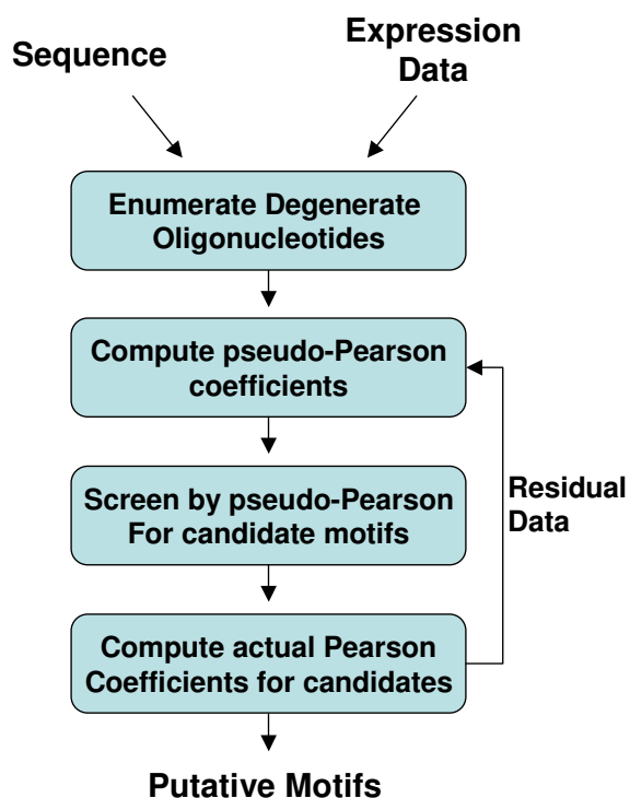
Figure 1 The fREDUCE algorithm. A set of possible IUPAC strings are generated from the input sequence. For each IUPAC string, we compute a pseudo-Pearson coefficient, which is an estimate and upper bound on the true Pearson coefficient. After the vast majority of motifs are filtered out using the pseudo-Pearson value, we then compute true Pearson coefficients for the remaining motifs and select the top motif. The residual expression value is then used to iteratively derive subsequent motifs.
