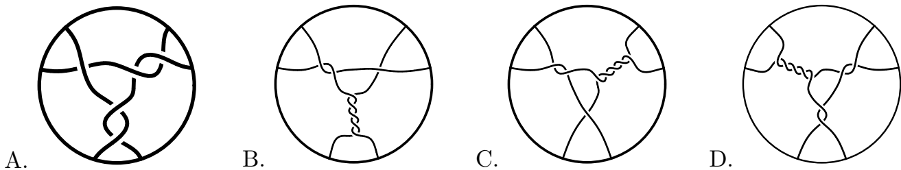
Figure 7 Three-branched supercoiled solutions to the tangle equations in Fig. 6.
