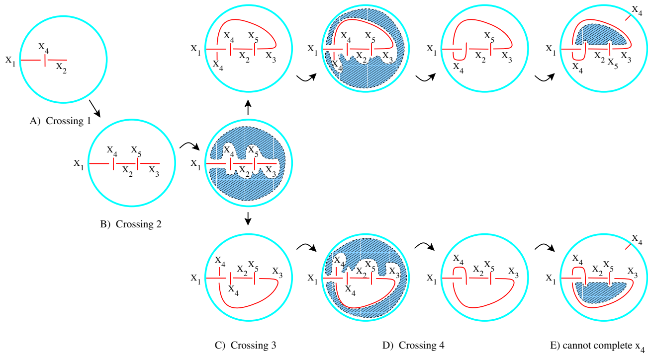
Figure 14 The matrix in Eqn. (4) does not correspond to a 3-string tangle.
