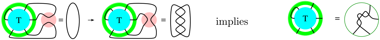
Figure 16 Solving for a 2-string tangle.
