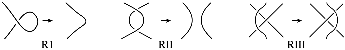
Figure 8 Reidemeister moves.
