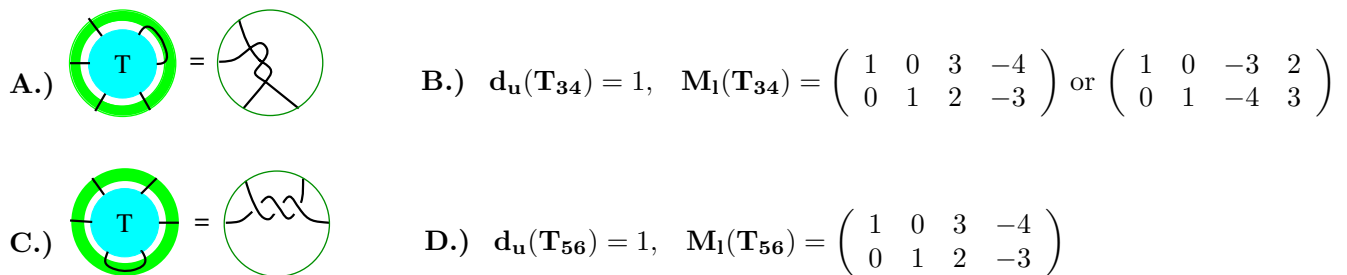
Figure 21 A.) The 2-string tangle T_{34} . This 2-string tangle is obtained from the 3-string tangle, T , by connecting endpoint arcs x_3 and x_4 . B.) The coloring invariants corresponding to the 2-string tangle T_{34} . C.) The 2-string tangle T_{56} . This 2-string tangle is obtained from the 3-string tangle, T , by connecting endpoint arcs x_5 and x_6 . D.) The coloring invariants corresponding to the 2-string tangle T_{56} .
