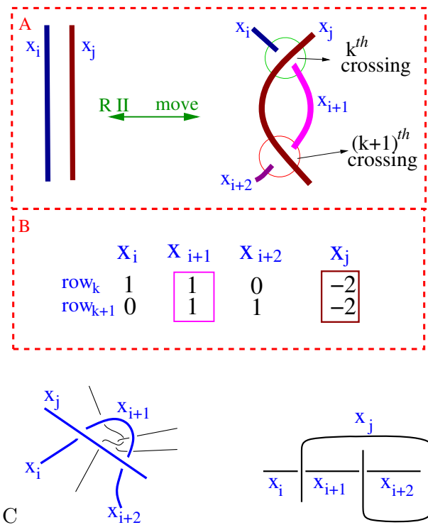
Figure 13 A.) An RII move. B.) Matrix corresponding to RII move. C.) Tangles which would also contain the submatrix in Fig. 13B.
