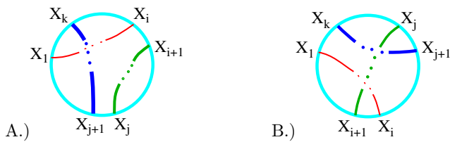
Figure 11 Possible parities. Note that the endpoint arcs are neither labeled consecutively nor in a clockwise fashion for tangle generation.
