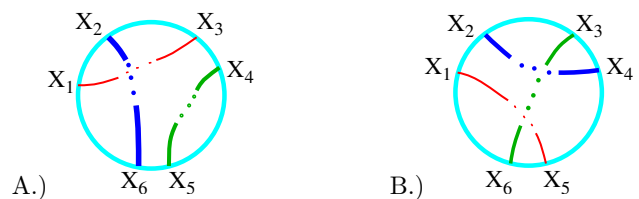
Figure 10 Possible parities.
