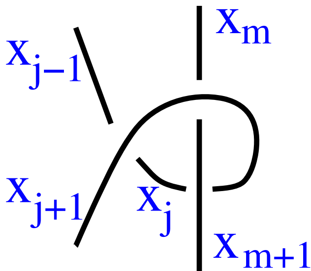
Figure 22 A diagram corresponding to Eqn. 9.
