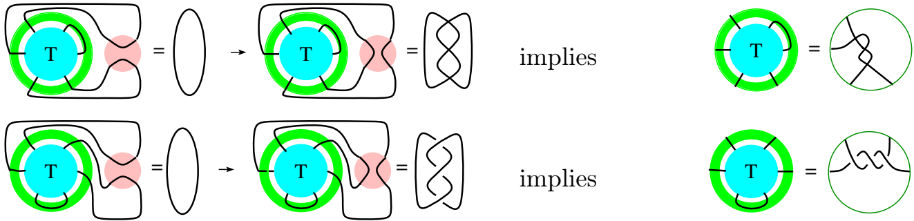
Figure 17 Solving for two more 2-string tangles.
