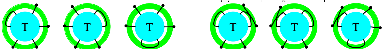
Figure 15 2-string tangle analysis will be used to determine these 2-string tangles from Fig. 6. The ends of the two strings are marked by dots.
