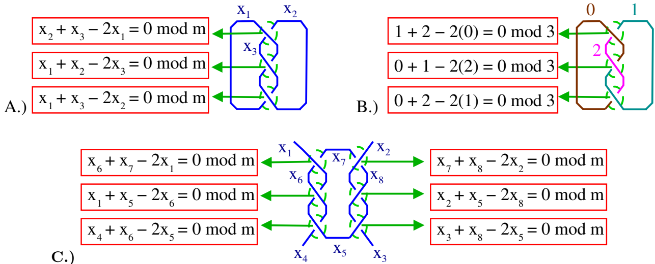
Figure 9 A.) Coloring a knot. The three arcs are labeled x_1, x_2, x_3 . A coloring of this knot diagram must satisfy the three equations corresponding to the three crossings. B.) A 3-coloring of this knot. C.) Coloring a 2-string tangle. The eight arcs are labeled x_1, x_2, \dots, x_8 . The six crossings result in six equations.
