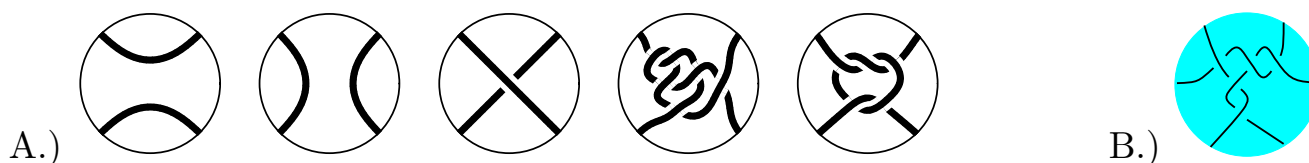
Figure 1 A.) Some 2-string tangles. B.) a 3-string tangle.
