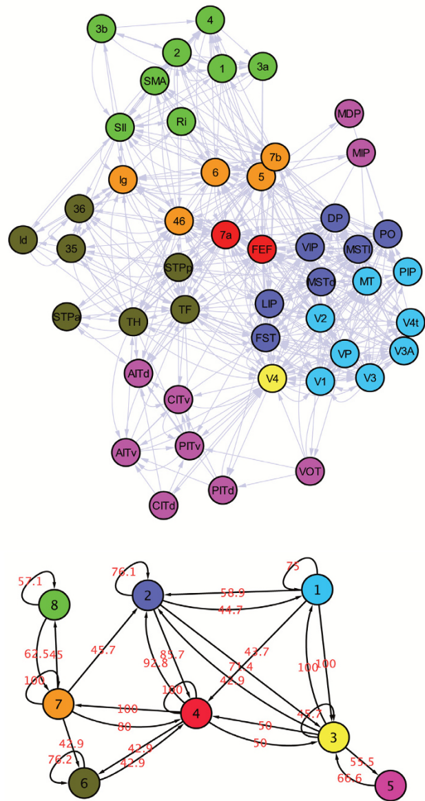
Figure 3 Macaque Cortex Network with 8 MixNet classes, with proportions. \hat{\alpha}_1 = 17.0 , \hat{\alpha}_2 = 14.9 , \hat{\alpha}_3 = 2.1 , \hat{\alpha}_4 = 4.3 , \hat{\alpha}_5 = 19.2 , \hat{\alpha}_6 = 14.9 , \hat{\alpha}_7 = 10.6 , \hat{\alpha}_8 = 17.0
